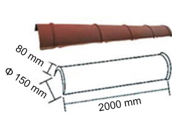
Circular Ridge Tile
