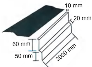
Draining Board
