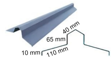
Ridge Tile With Angle
