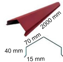
Ridge Tile With Angle
