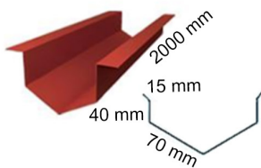
Gutter Bed
