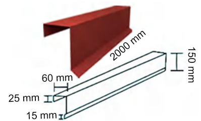
Gable Board
