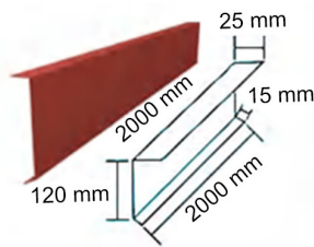
Cornice
