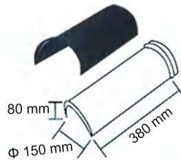
380 Circular Ridge Tile
